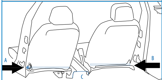
Seat bottom frame structural tubes - A, B Center floor tunnel-mounted crush box - C
