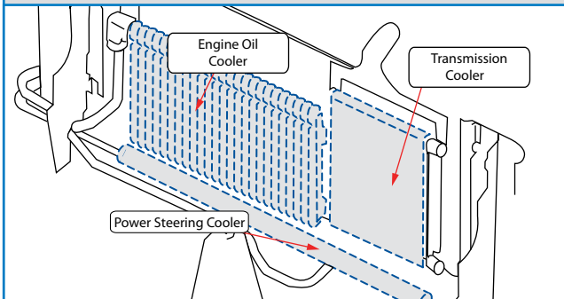
Three auxiliary air-to-oil coolers are mounted in front of the engine coolant radiator. The transmission cooler is connected in series with the coolant radiator end-tank cooler.
